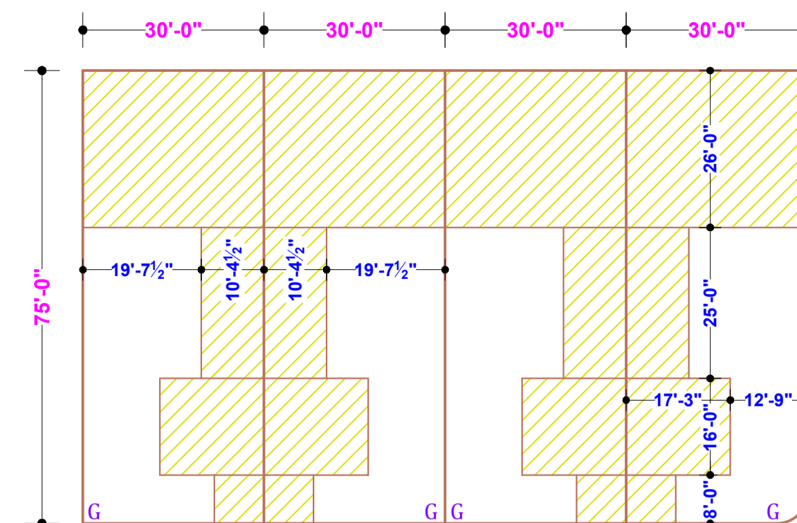
ZONING PLAN FOR 250 SQ. YARDS PLOTS
